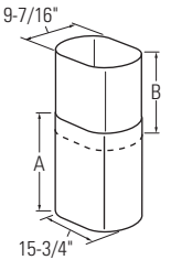
ZV850 Duct Cover Dimensions
